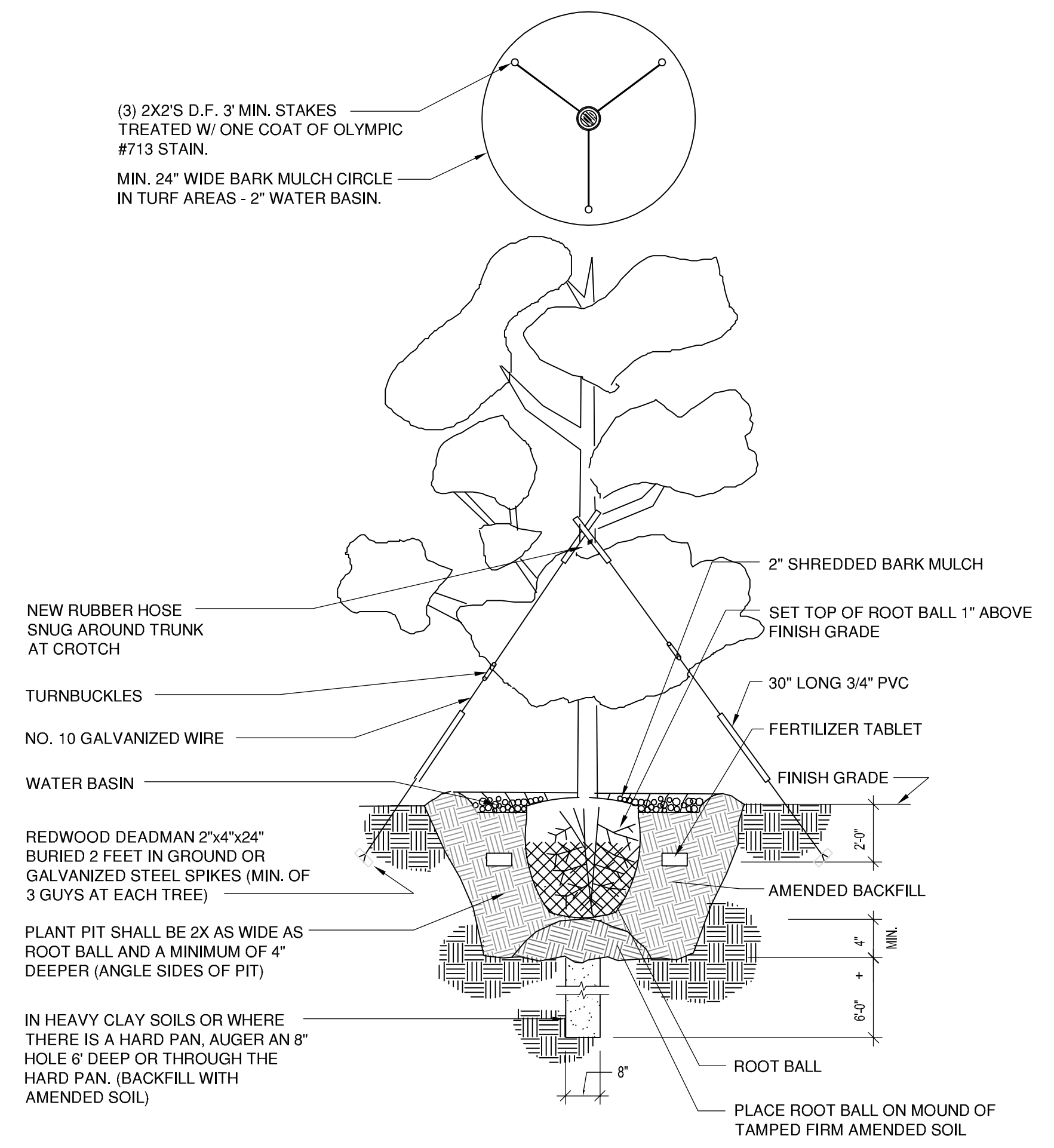
EVERGREEN TREE PLANTING DETAIL
